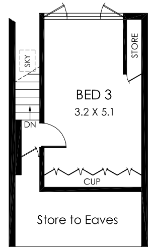
LEVEL 3
