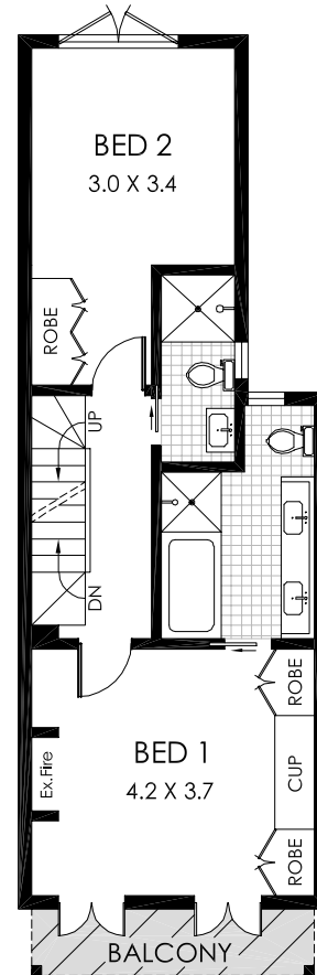
LEVEL 2
